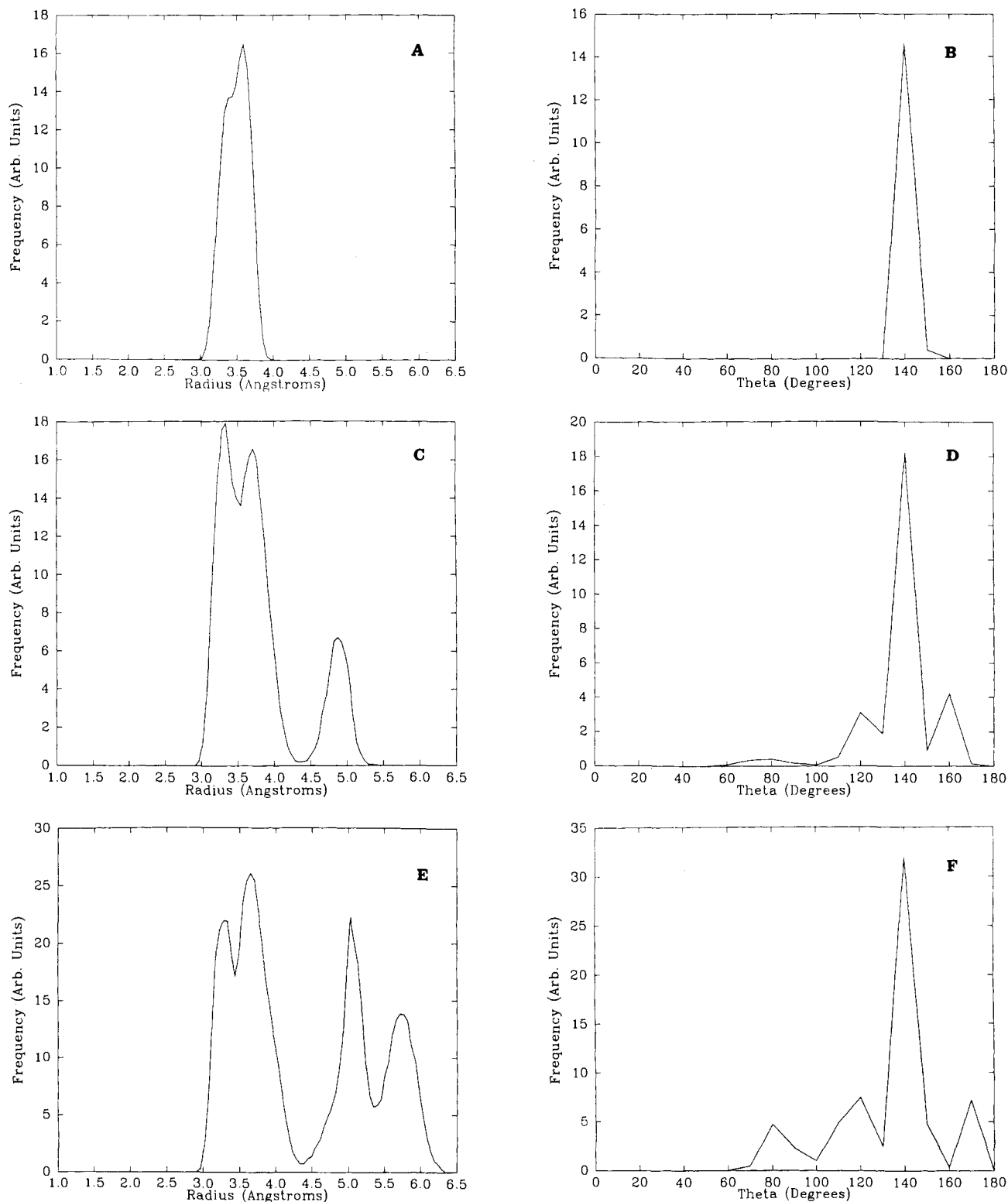
Figure 5. Radial and \theta histograms of the water distributions at R_{\text{NO}_2^-\text{Li}^+} = 3 \text{ \AA} (For radial histograms, arbitrary units = frequency \times 10^4 ; for \theta histograms, arbitrary units = frequency \times 10^5 ): (A) radial histograms for n = 3 cluster, (B) \theta histogram for n = 3 cluster, (C) radial histogram for n = 5 cluster, (D) \theta histogram for n = 5 cluster, (E) radial histogram for n = 9 cluster, and (F) \theta histogram for n = 9 cluster.
